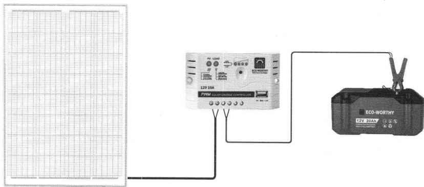
(10W Solar panel kit)
